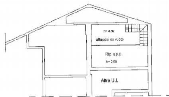
PIANO SOPPALCO
